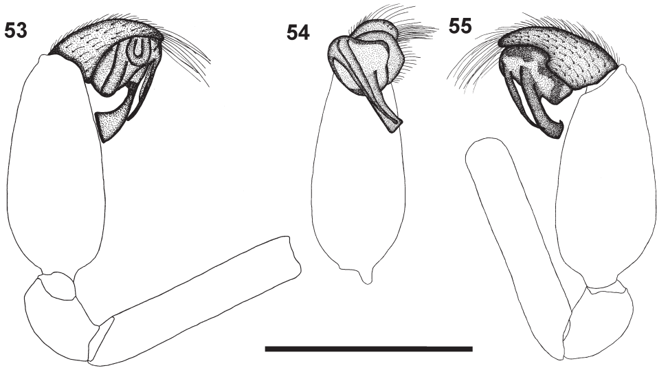
Figures 53–55. Left palp of male Calommata megae sp. n. 53 prolateral view 54 ventral view 55 retrolateral view. Scale bars: 1mm.
