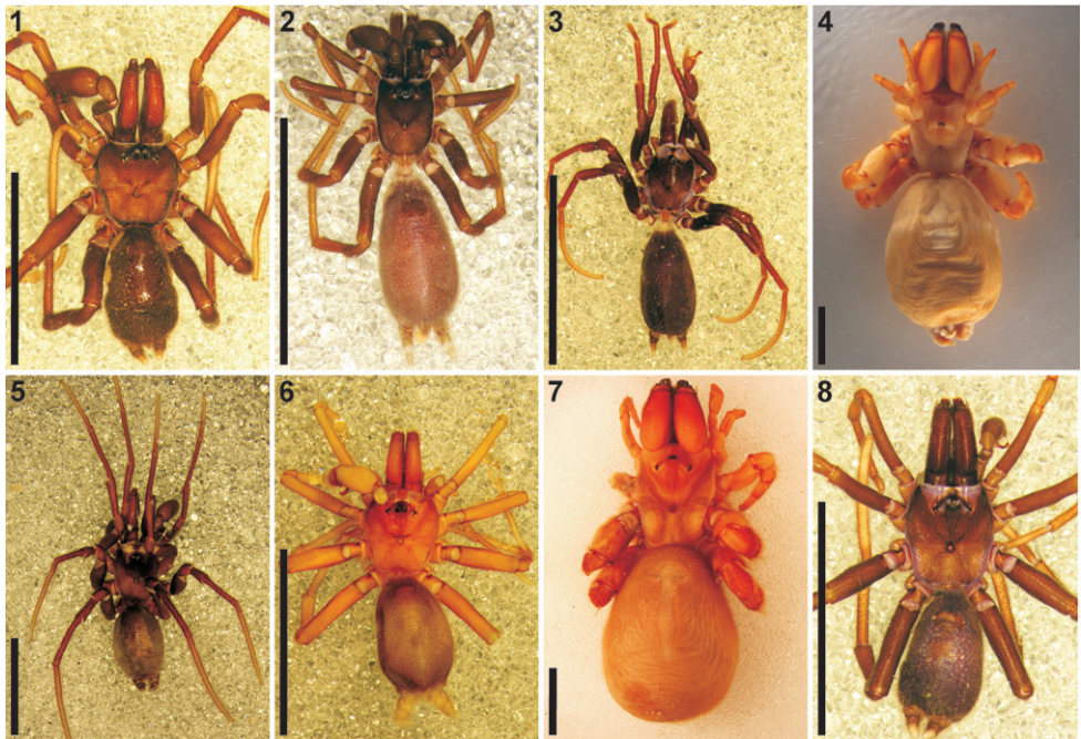
Figures 1–8. Dorsal habitus of Afrotropical Calommata species 1 C. megae sp. n., male (Harare, Zimbabwe) 2 C. meridionalis sp. n., male (Erferis Dam, South Africa) 3 C. namibica sp. n., male (Etosha, Namibia) 4 C. simoni Pocock, female (Galim, Cameroon) 5 same, male (Dja Reserve, Cameroon) 6 C. tibialis sp. n., male (Bassari–Sokodé, Togo) 7 C. transvaalica Hewitt, female (Blouberg, South Africa) 8 same, male (Groenkloof, South Africa). Scale bars: 5mm.
