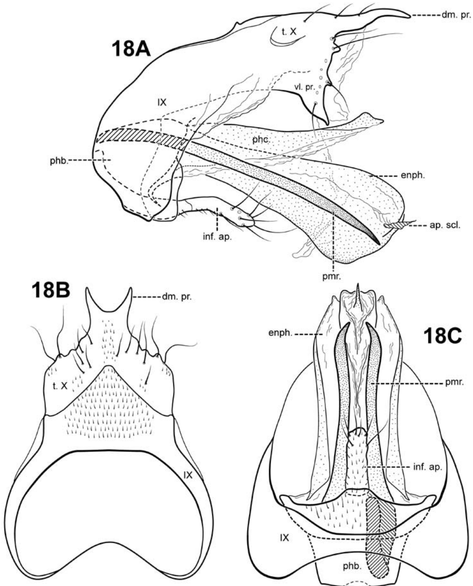
Figure 18. Itauara peruensis , sp. n. (UMSP000210957). Male genitalia A lateral B dorsal C ventral. Abbreviations: ap. scl. = apical sclerite; dm. pr. = dorsomesal process; enph. = endophallus; inf. ap. = inferior appendage process; phb. = phallobase; phc. = phallicata; pmr. = paramere; t. X = tergum X; vl. pr. = ventrolateral process.
