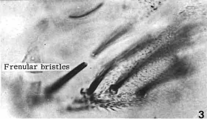
FIGS. 1-3. Parasabatinca aftimacrai spec. nov., 1. holotype, 2. apex of forewing, 3. costal margin with frenular bristles; all specimens in lebanese amber.
