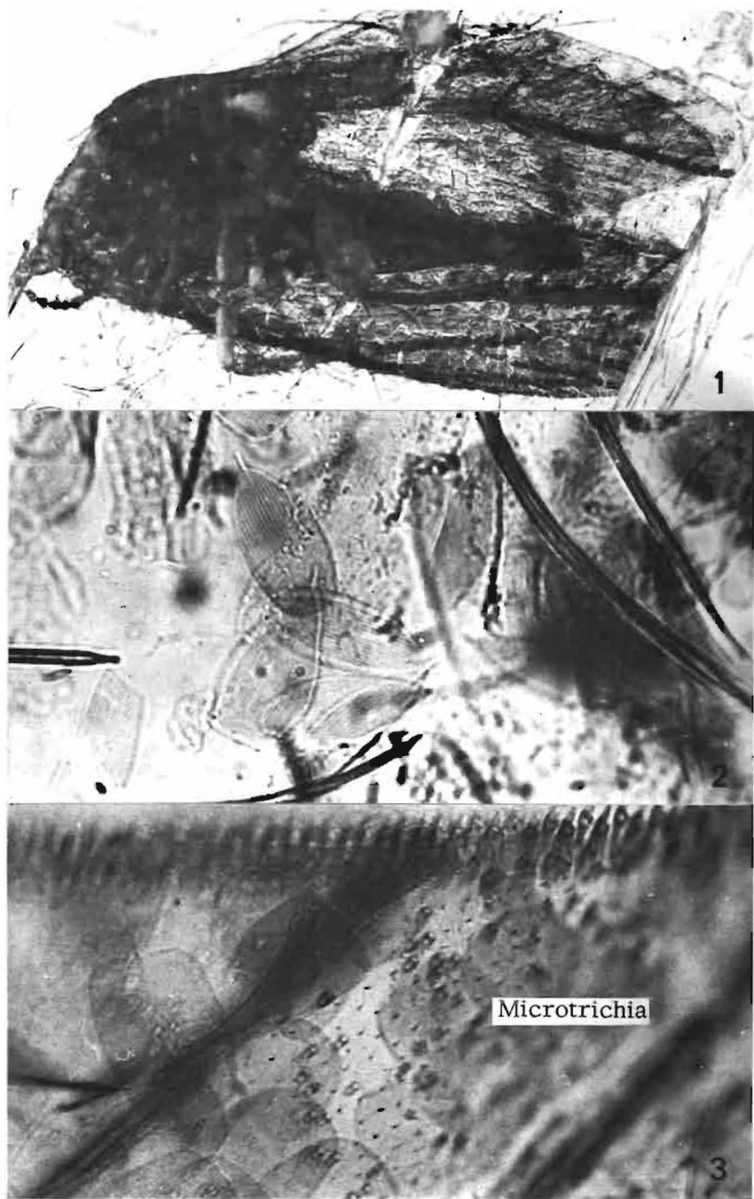
FIGS. 1-3. Parasabatinca astimacrai spec. nov., 1. paratype, 2. scales on forewing, 3. scales and microtrichia on forewing; all specimens in lebanese amber.
