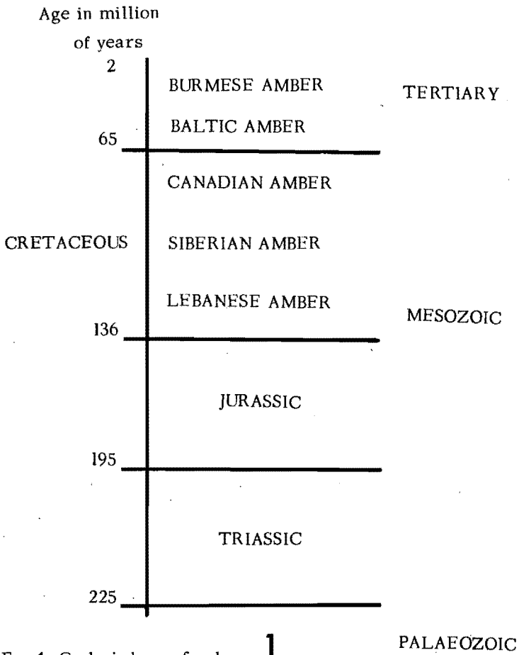
FIG. 1. Geological age of ambers.
