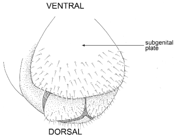
Fig. 4. Ventral habitus of Sphaeropsocus kuenowii Hagen (KU B-148), with detail of compound eye and terminal sternites.
