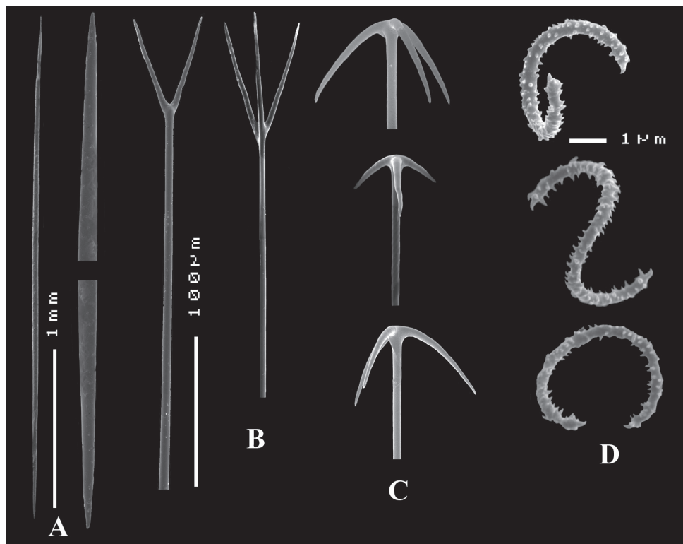
Fig. 3. Cinachyrella arabica (Carter, 1869), ZMA Por. 14608, A, oxeas, B, prodiaene and protriaene, C, anatriaenes, D, sigmaspires.
